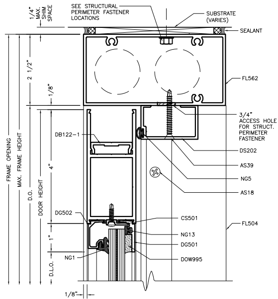
C.O.C. TRANSOM BAR W/ OFFSET ARM 1:2
