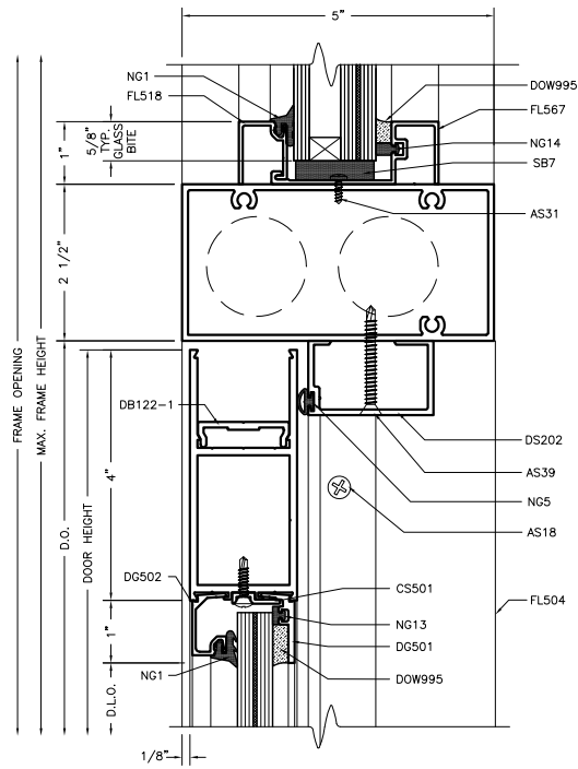
C.O.C. DOOR FRAME HEADER W/ OFFSET ARM 1:2
