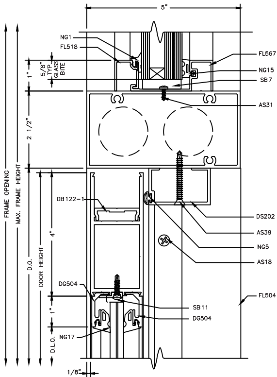
C.O.C. DOOR FRAME HEADER W/ OFFSET ARM 1:2
