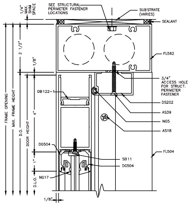
C.O.C. TRANSOM BAR W/ OFFSET ARM 1:2
